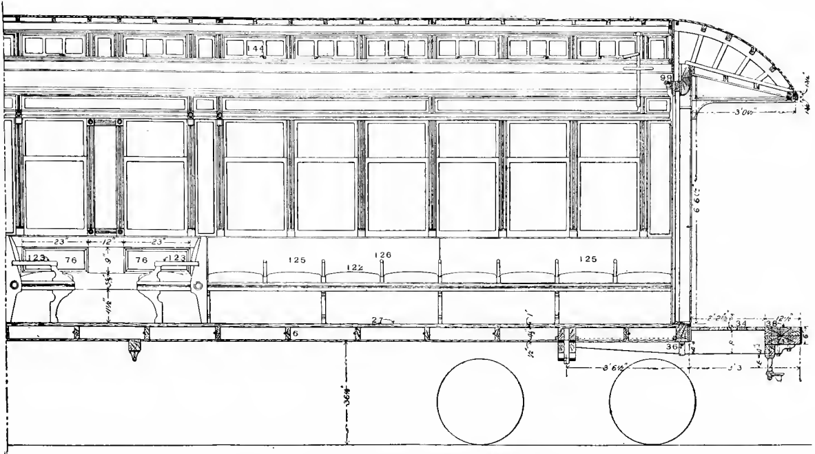
Fig. 464. Half Longitudinal Section, Showing Interior.
